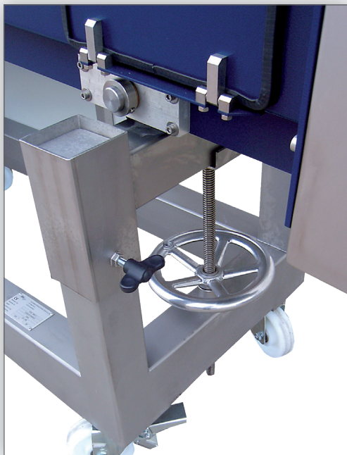
Independent height adjustment facilities, mounted both on the strand die head and pelletizer side of the machine sub-frame
